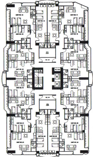
TYPICAL 5TH - 14TH FLOOR PLAN
